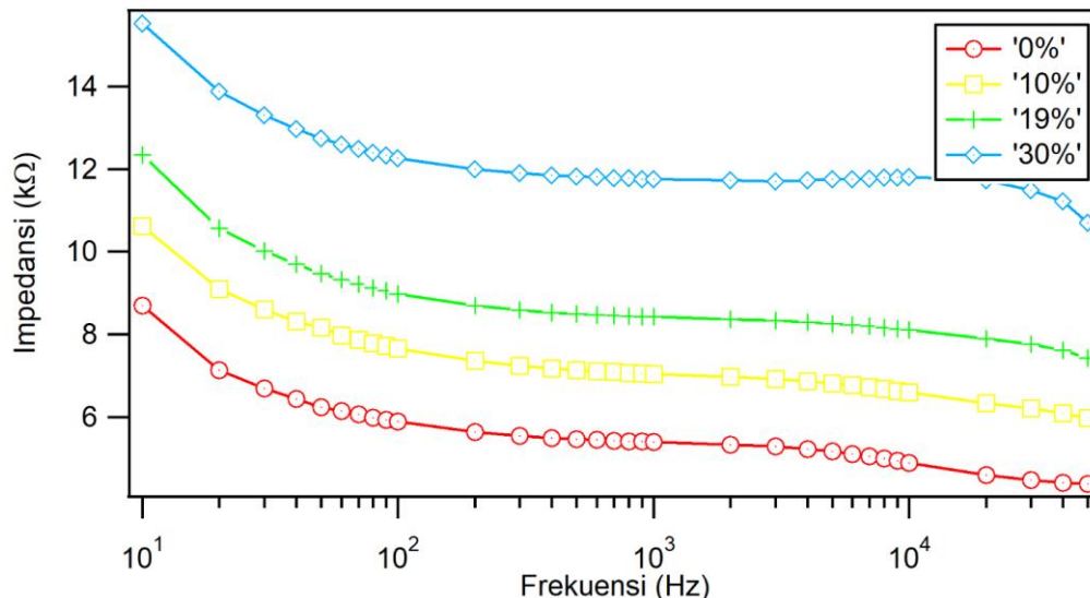
FIGURE 4. Results of impedance measurements on sugar solution composing fruit sweetness.
