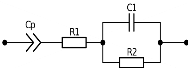
FIGURE 1. The equivalent circuit of solution.
